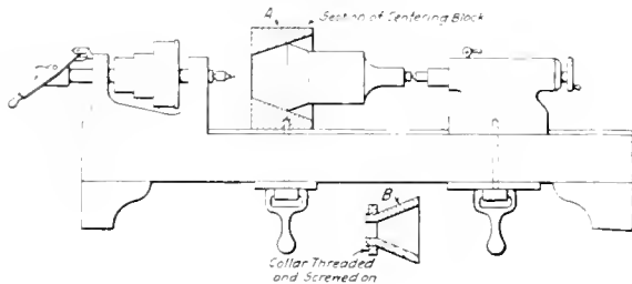
Centering Machine Developed from an Old Lathe
